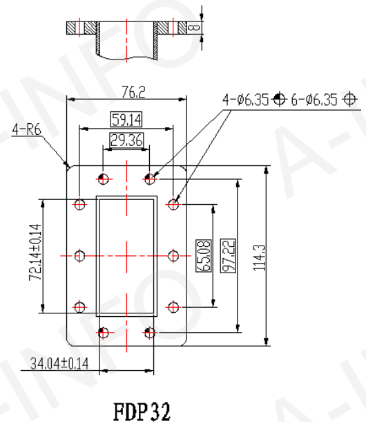
Flange Drawing
