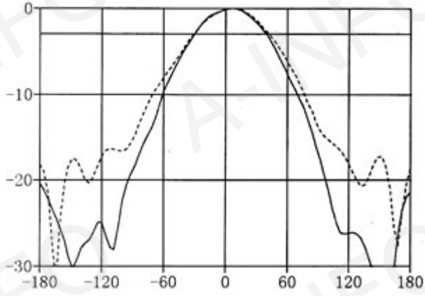
Frequency: 3.2GHz
