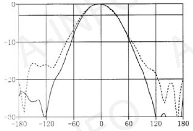
Frequency: 3.6GHz
