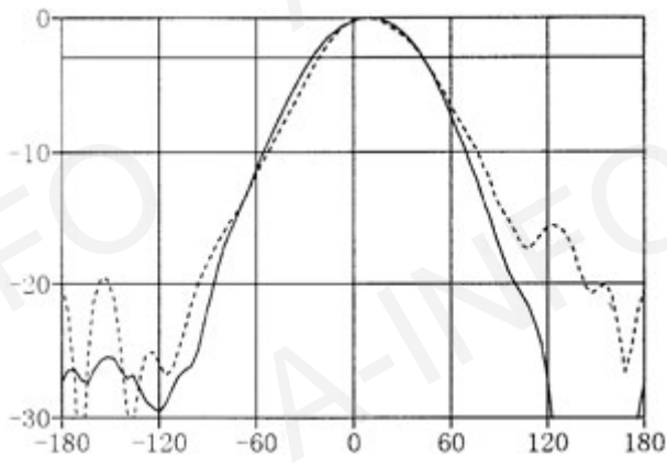
Frequency: 4.0GHz
