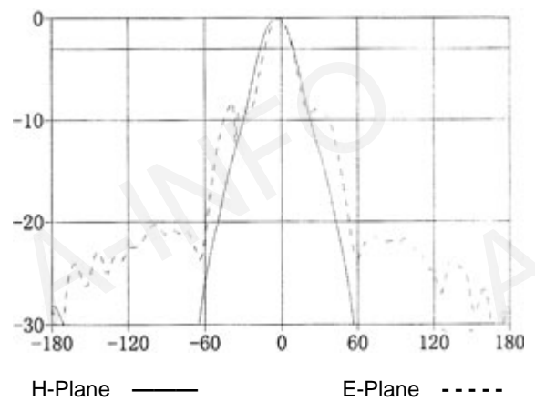
Frequency: 3.5GHz
