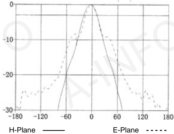
Frequency: 3.0GHz
