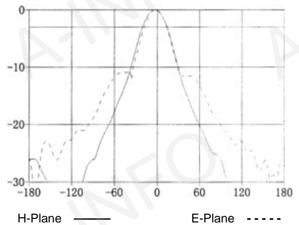
Frequency: 2.5GHz
