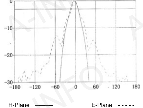
Frequency: 4.5GHz
