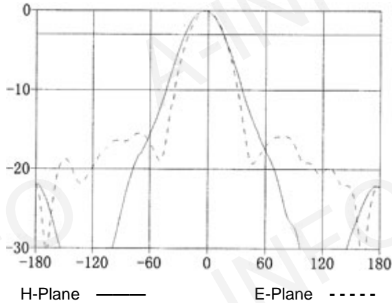
Frequency: 2.0GHz
