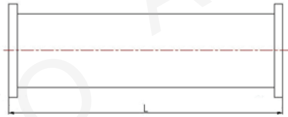
Standard Models
